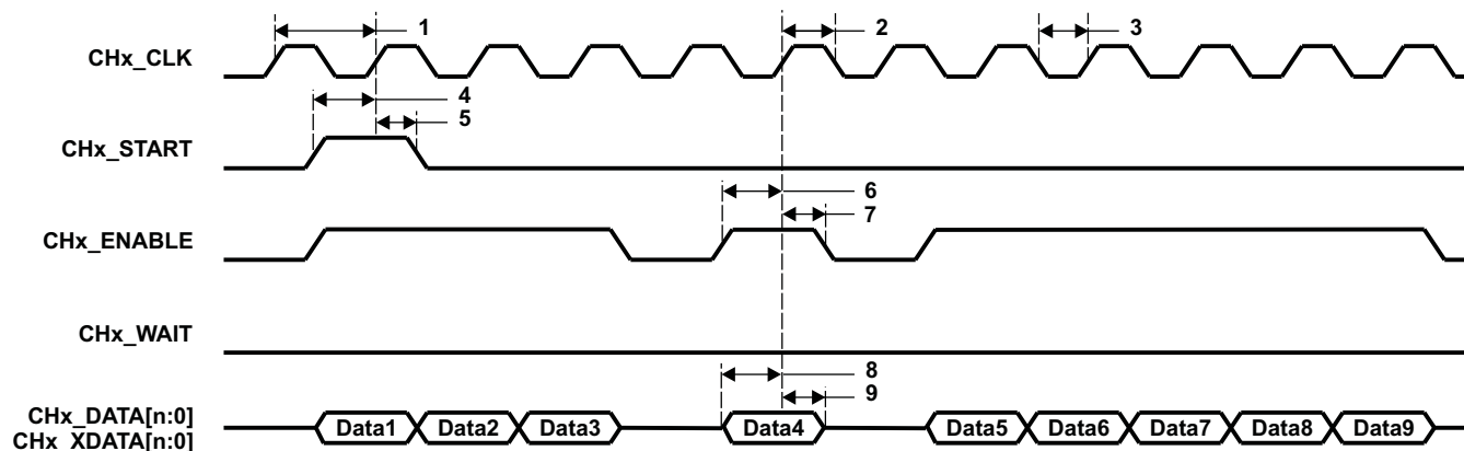
Figure 6-57. uPP Single Data Rate (SDR) Receive Timing
