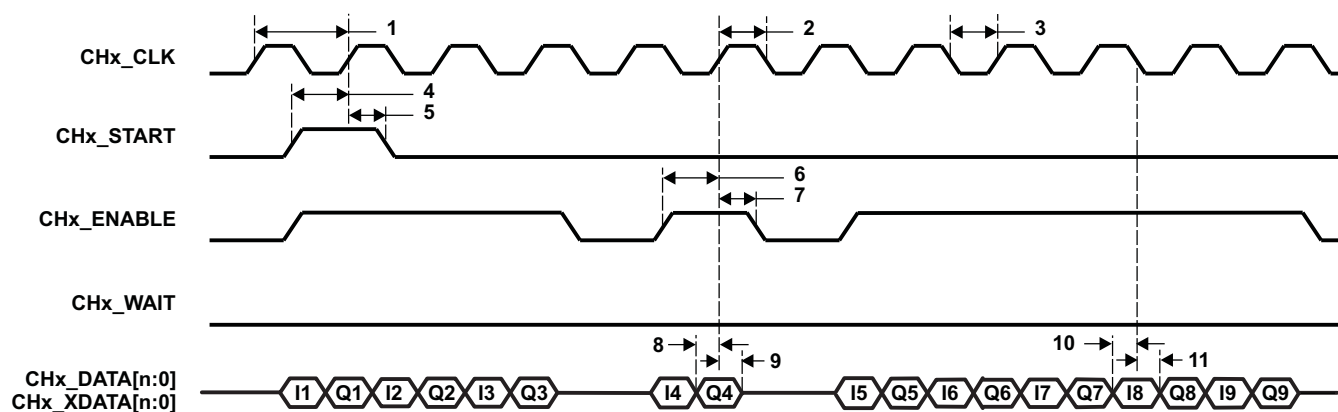
Figure 6-58. uPP Double Data Rate (DDR) Receive Timing
