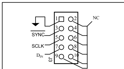
Figure 3: J3 Serial Interface Header
