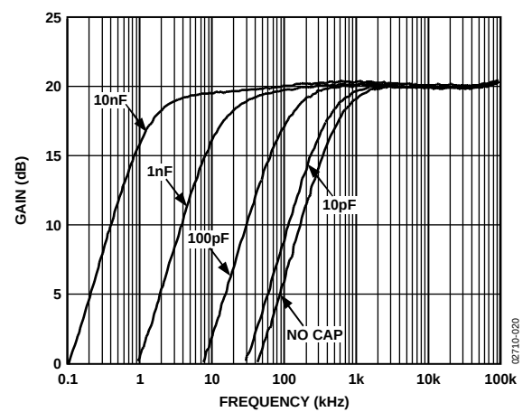
Figure 20. Gain vs. Frequency for Multiple Values of HPFL Capacitor at V_{GAIN} = 500 mV
