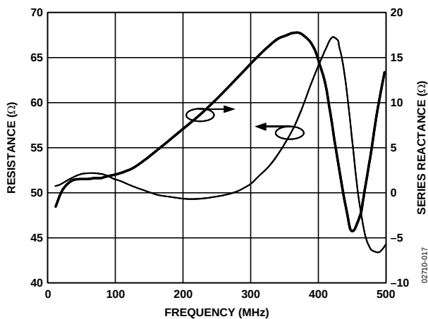
Figure 17. Output Resistance and Series Reactance vs. Frequency at V_{GAIN} = 500 mV
