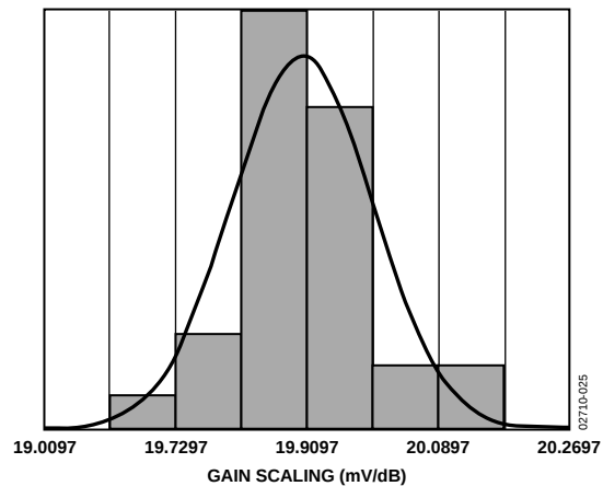
Figure 25. Gain Scaling Distribution at 70 MHz
