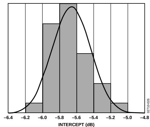
Figure 26. Gain Intercept Distribution at 70 MHz
