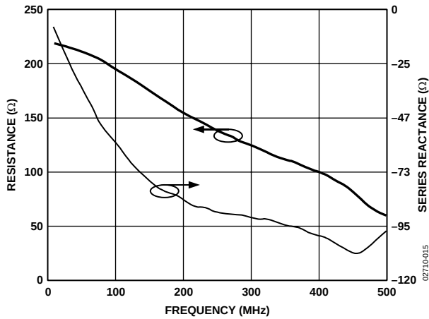
Figure 15. Input Resistance and Series Reactance vs. Frequency at V_{GAIN} = 500 mV
