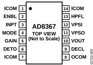
Figure 2. Pin Configuration
