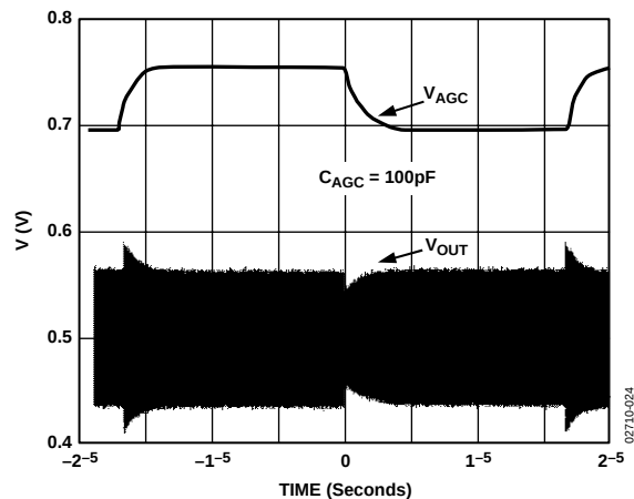
Figure 24. AGC Time Domain Response (3 dB Step)
