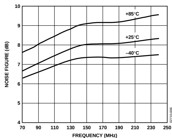
Figure 6. NF (re 200\ \Omega ) vs. Frequency at Maximum Gain
