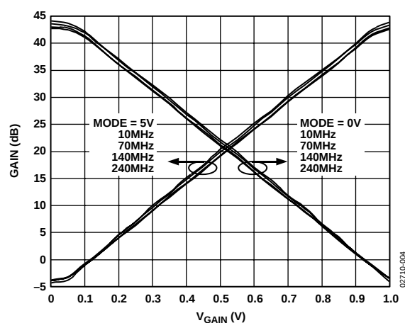
Figure 4. Gain vs. V_{\text{GAIN}} (Mode LO and Mode HI)
