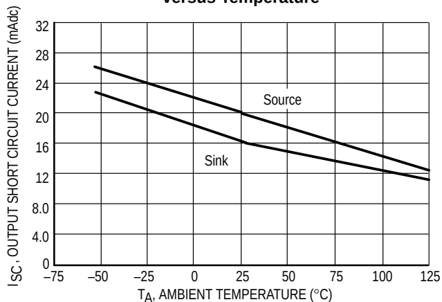
Figure 7. Output Short Circuit Current versus Temperature
