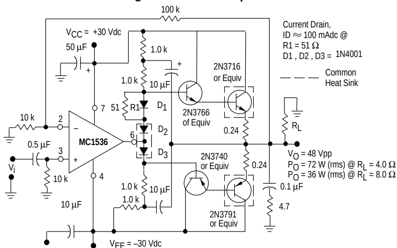
Figure 11. Audio Amplifier
