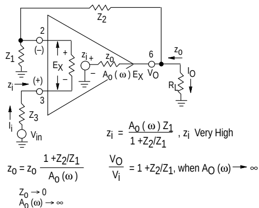
Figure 10. Noninverting Feedback Model
