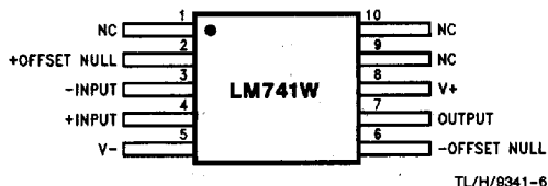
Ceramic Flatpak
