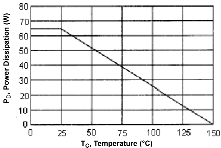
Power Derating
