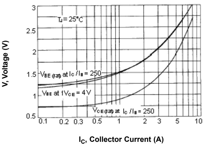
Figure - 9 "ON" Voltage
