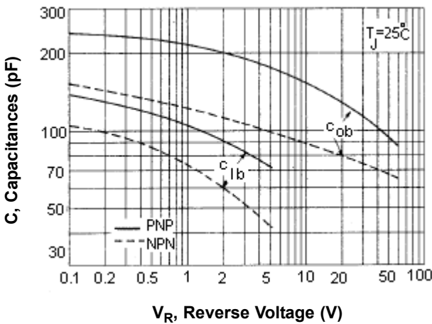
Figure - 5 Capacitances
