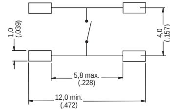
PAD LAYOUT
