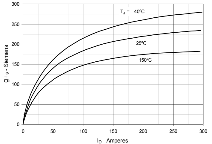
Fig. 8. Transconductance
