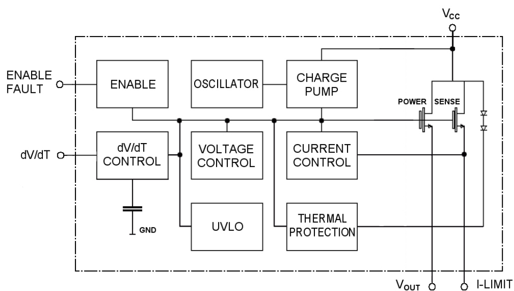
Figure 1. Block diagram
