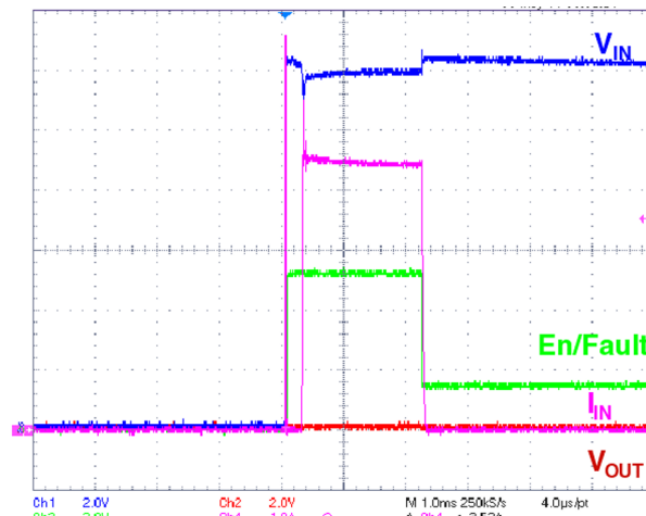
Figure 20. Startup into output short-circuit (fast rise)
