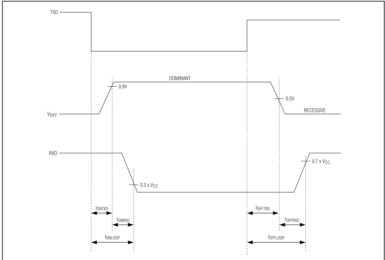
Figure 1. Timing Diagram
