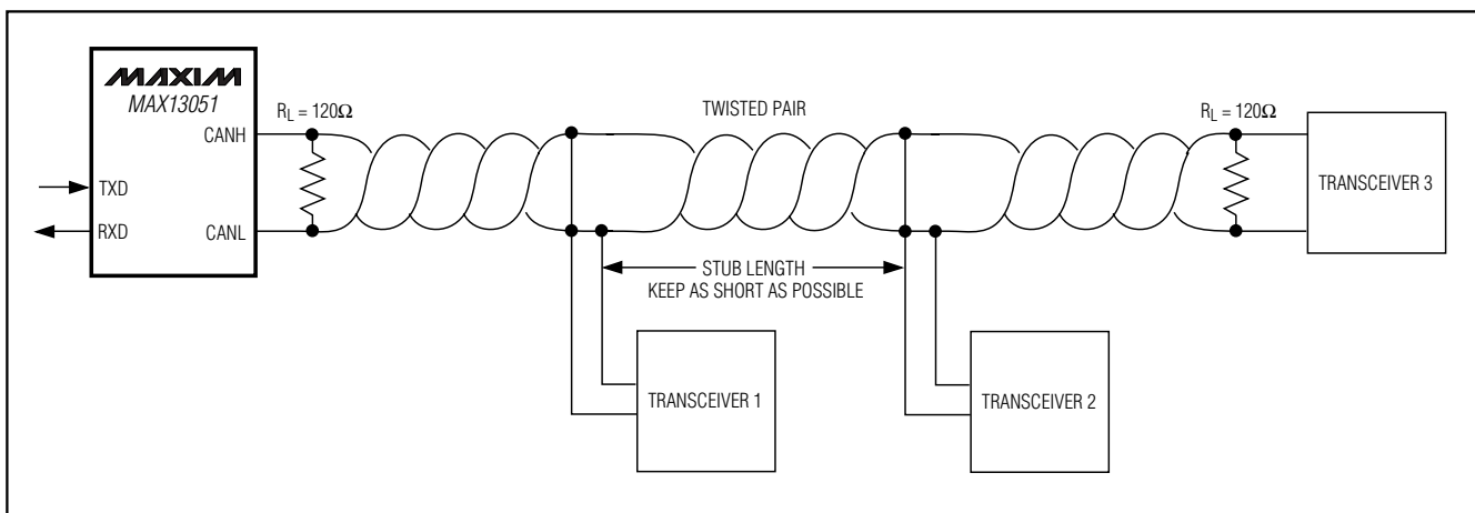
Figure 6. Multiple Receivers Connected to CAN Bus
