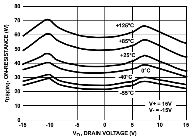
FIGURE 2. \pm 15\text{V} DUAL SUPPLY r_{\text{ON}} CURVES AT VARIOUS TEMPERATURES
