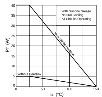
Pr-Ta Characteristics
