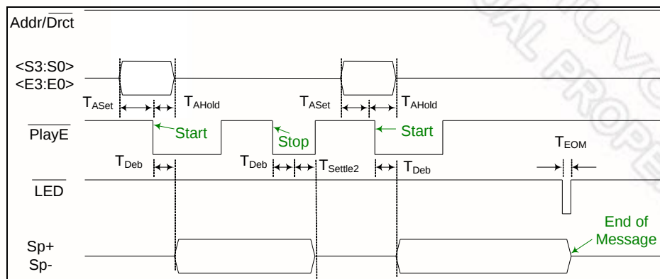
Figure 6-4 Playback-Edge ( \overline{\text{PlayE}} ) function
