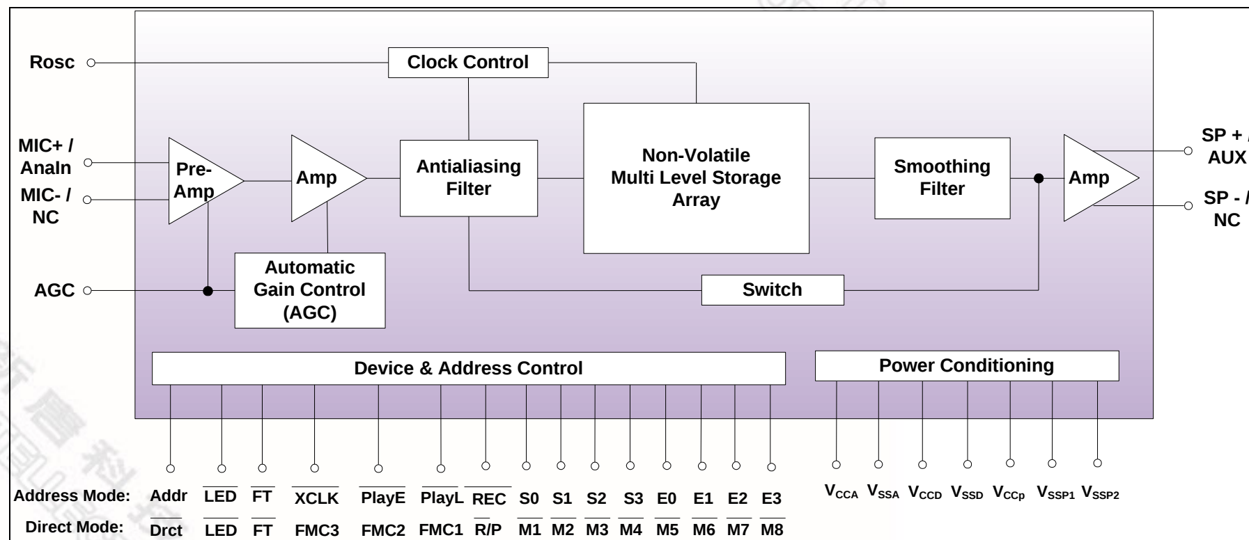
Figure 3-1 Block Diagram
