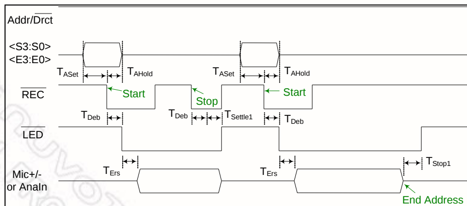
Figure 6-3 Record-Edge ( \overline{\text{REC}} ) function with on-off
