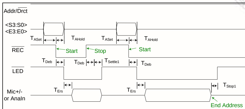
Figure 6-2 Record-Level ( \overline{\text{REC}} ) function with start and stop actions
