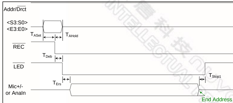
Figure 6-1 Record-Level ( \overline{\text{REC}} ) function till end address
