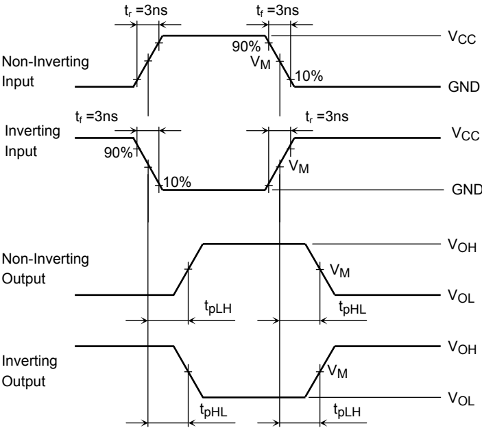
Figure 2 t_{pLH} , t_{pHL}
