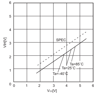
Fig.6 "H" input voltage V_{IH}(V_{CC}, SCK, SI, HOLD, WP)
