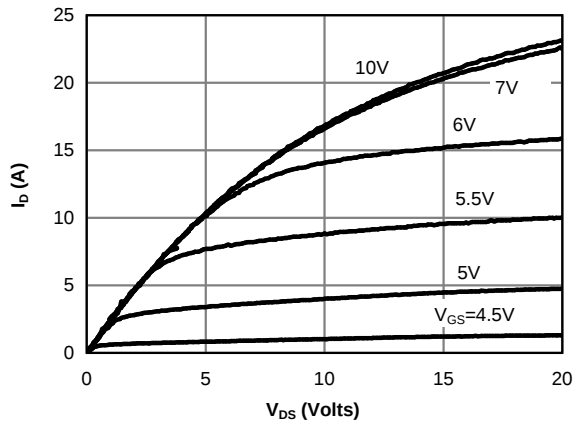
Figure 1: On-Region Characteristics@25°C
