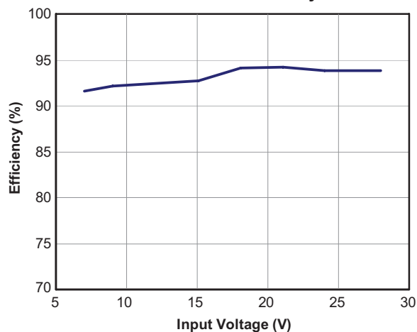
Electrical Efficiency
