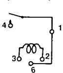
1 FORM A (SPST-NO)
