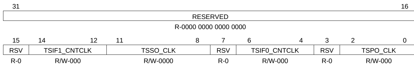
Figure 4-3. TSIFCTL Register [0x01C4 0050]
