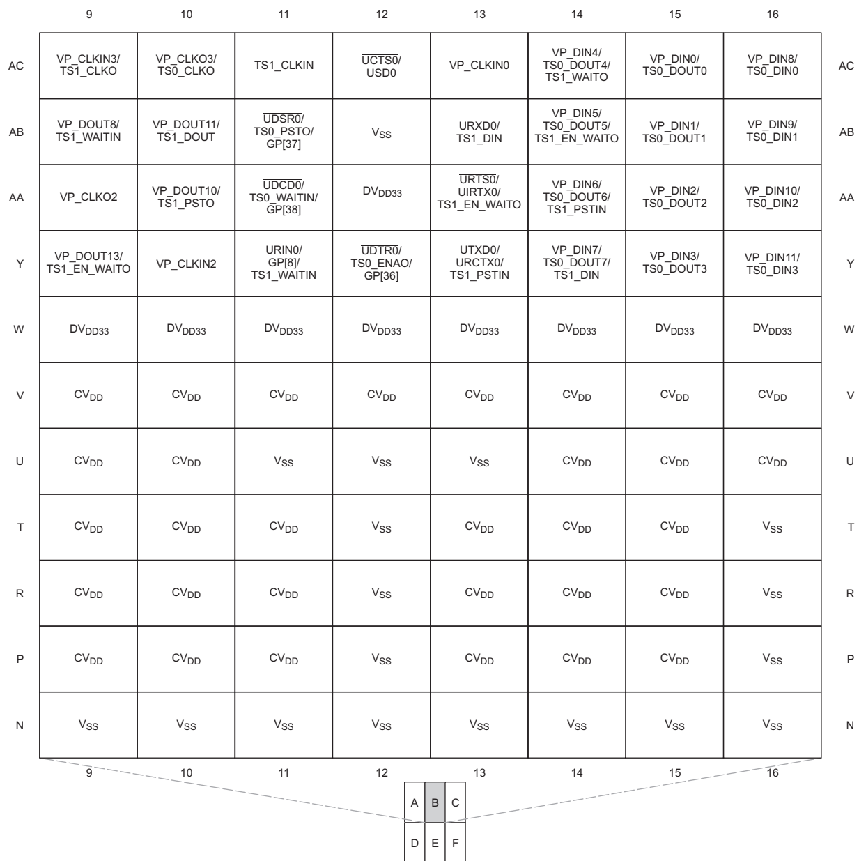
Figure 3-3. Pin Map [Section B]
