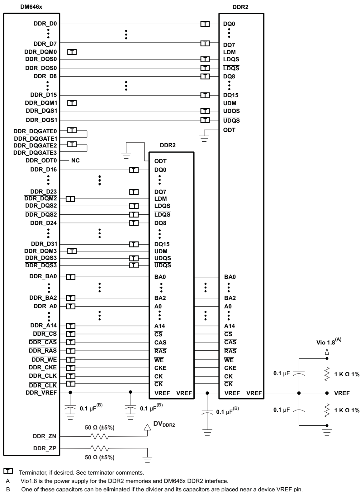
Figure 7-27. DM6467 32-Bit DDR2 High Level Schematic
