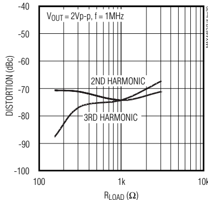
MAX4352/MAX4353/MAX4354 DISTORTION vs. OUTPUT RESISTANCE
