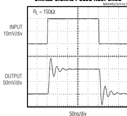
MAX4352/MAX4353/MAX4354 SMALL-SIGNAL PULSE RESPONSE
