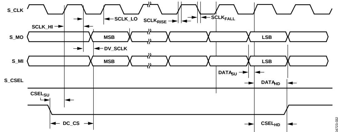
Figure 23. SPI Port—Input Timing
