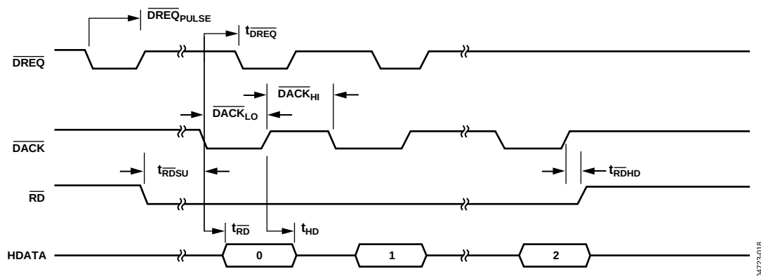
Figure 9. Single Read for DREQ/DACK DMA Mode for Assigned DMA Channel (EDMOD0/EDMOD1 <14:11> NOT Programmed to a Value of 0000)
