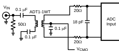
Figure 34. Low Input Frequency Transformer Drive Circuit
