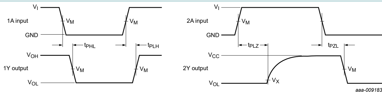
Fig. 7. The data input 1A to output 1Y and input 2A to output 2Y propagation delays
