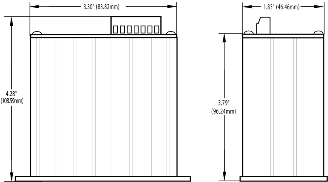
Dimensions—SNAP PAC Serial Brains
