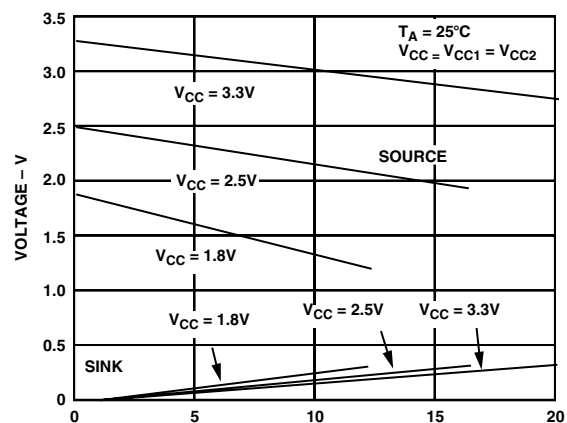
TPC 23. Y Sink and Source Current
