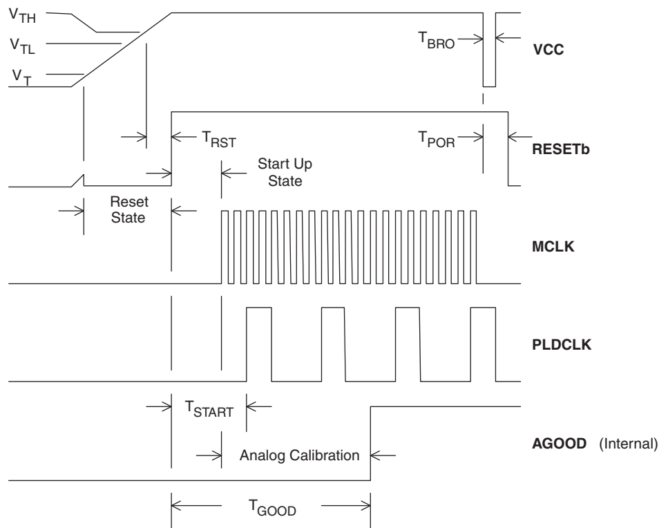
Figure 2. ispPAC-POWR1220ATE Power-On Reset
