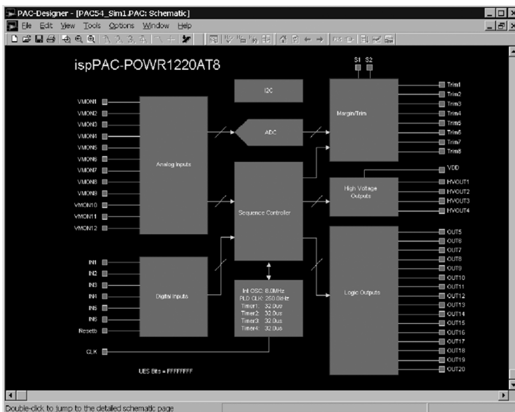
Figure 33. PAC-Designer ispPAC-POWR1220AT8 Design Entry Screen
