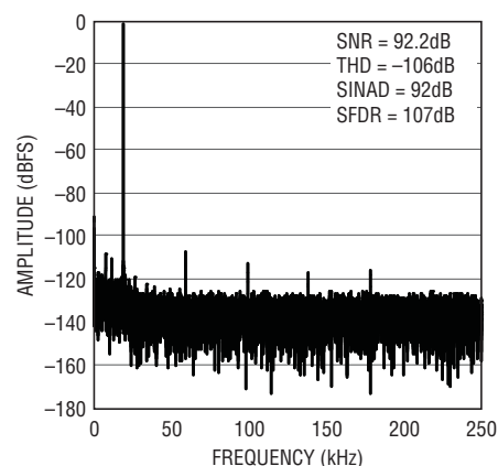
32k Point FFT f_s = 500\text{ksps} , f_{\text{IN}} = 20\text{kHz}
