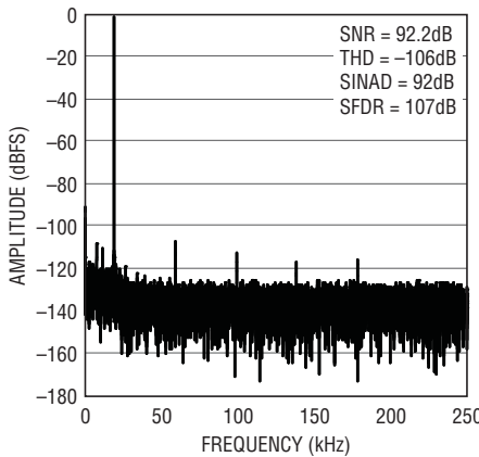
32k Point FFT f_S = 500\text{Kpsps} , f_{IN} = 20\text{kHz}
