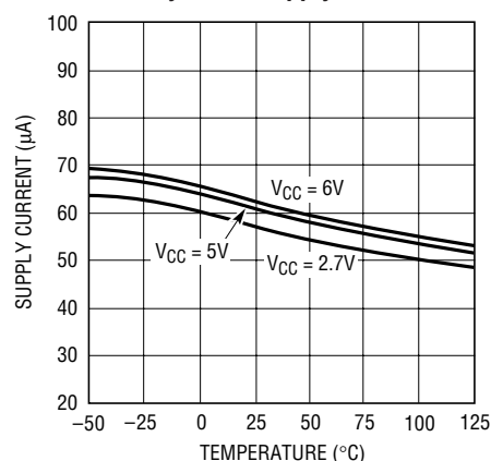
Standby Mode Supply Current
