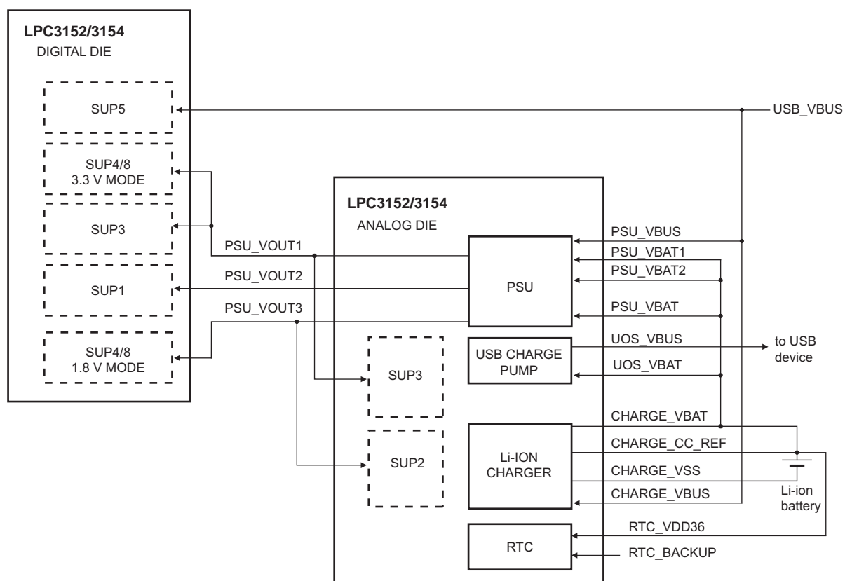
Fig 13. LPC3152/3154 supply voltages of the analog and digital die
