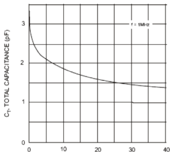
V_R , REVERSE VOLTAGE (V) Fig. 3 Typical Capacitance
