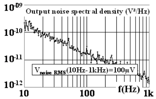
Figure 8: S_{\text{Vout}}(\text{V}^2/\text{Hz}) @ 25^{\circ}\text{C} , I_{\text{Load}}=100\text{mA}
