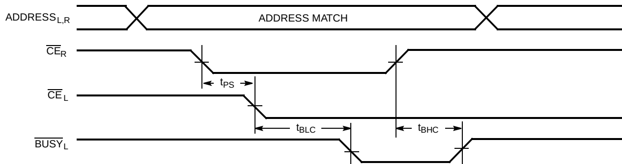
Busy Timing Diagram No. 2 (Address Arbitration) [36] Left Address Valid First:
