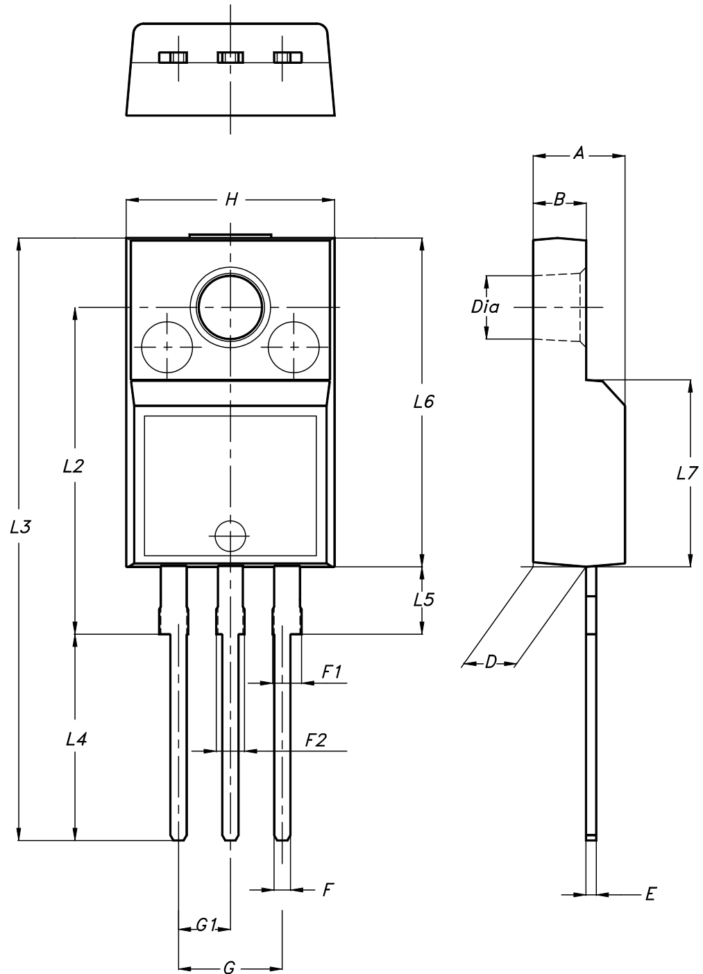
Figure 39. TO-220FP package outline
