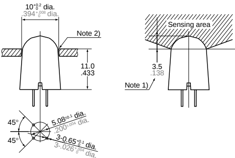
Recommended PC board pattern (BOTTOM VIEW)
