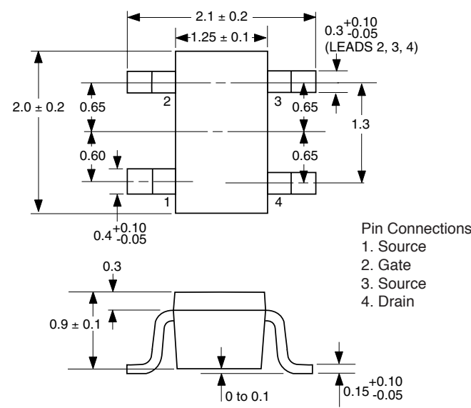
PACKAGE OUTLINE 18
