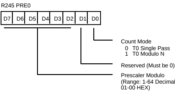
Figure 56. Prescaler 0 Register (F5 H : Write-Only)
