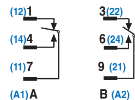
INPUT ON DELAY
