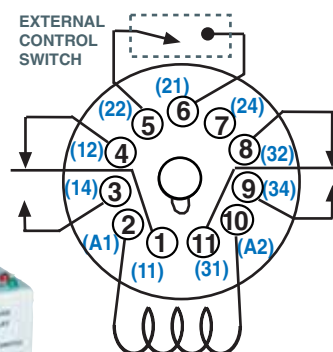
INPUT OFF DELAY
