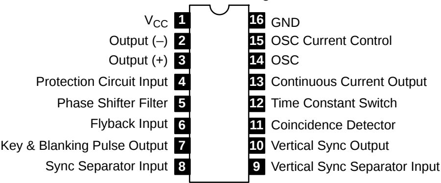
Pin Connection Diagram
