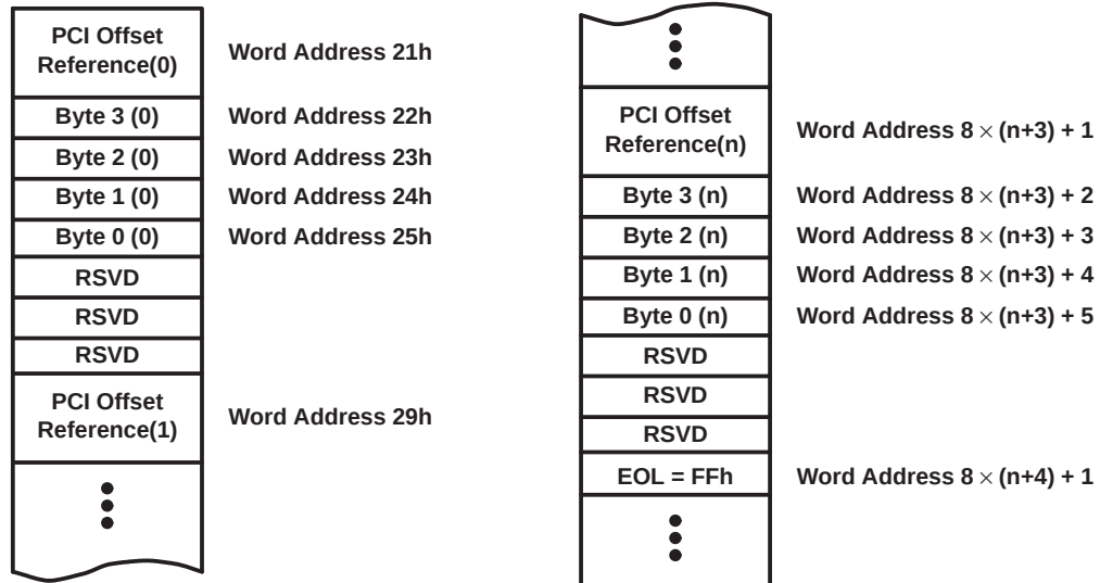
Figure 3-7. EEPROM Data Format
