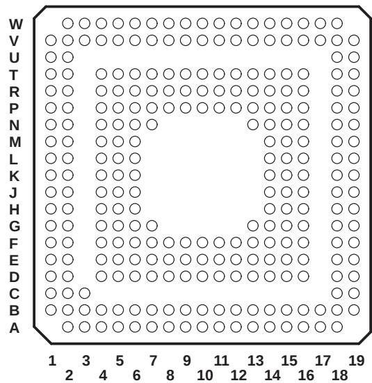
Figure 2-1. PCI1451 GJG Terminal Diagram
