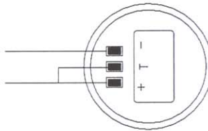
Connection diagram
