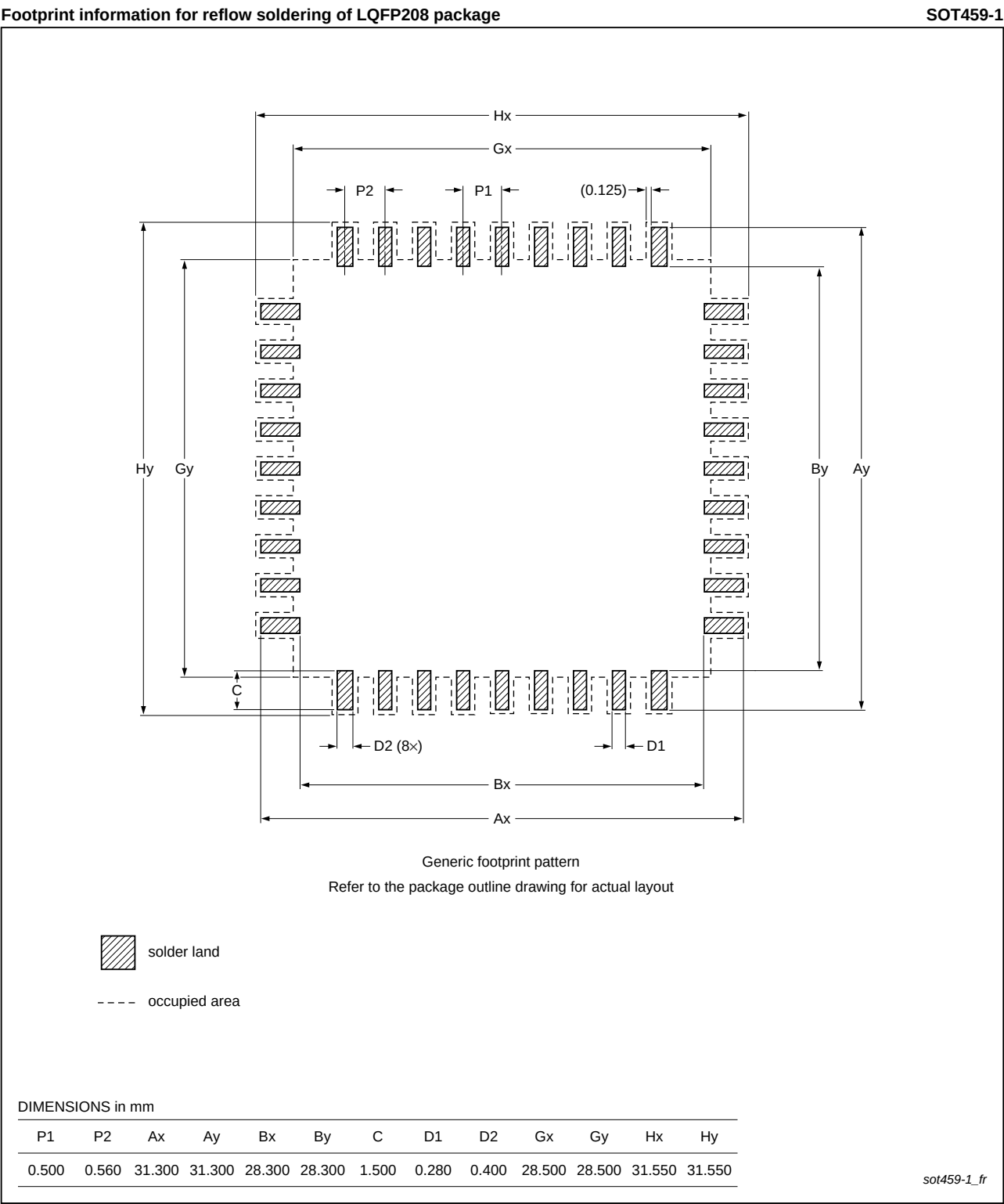
Fig 50. Reflow soldering of the LQFP208 package
