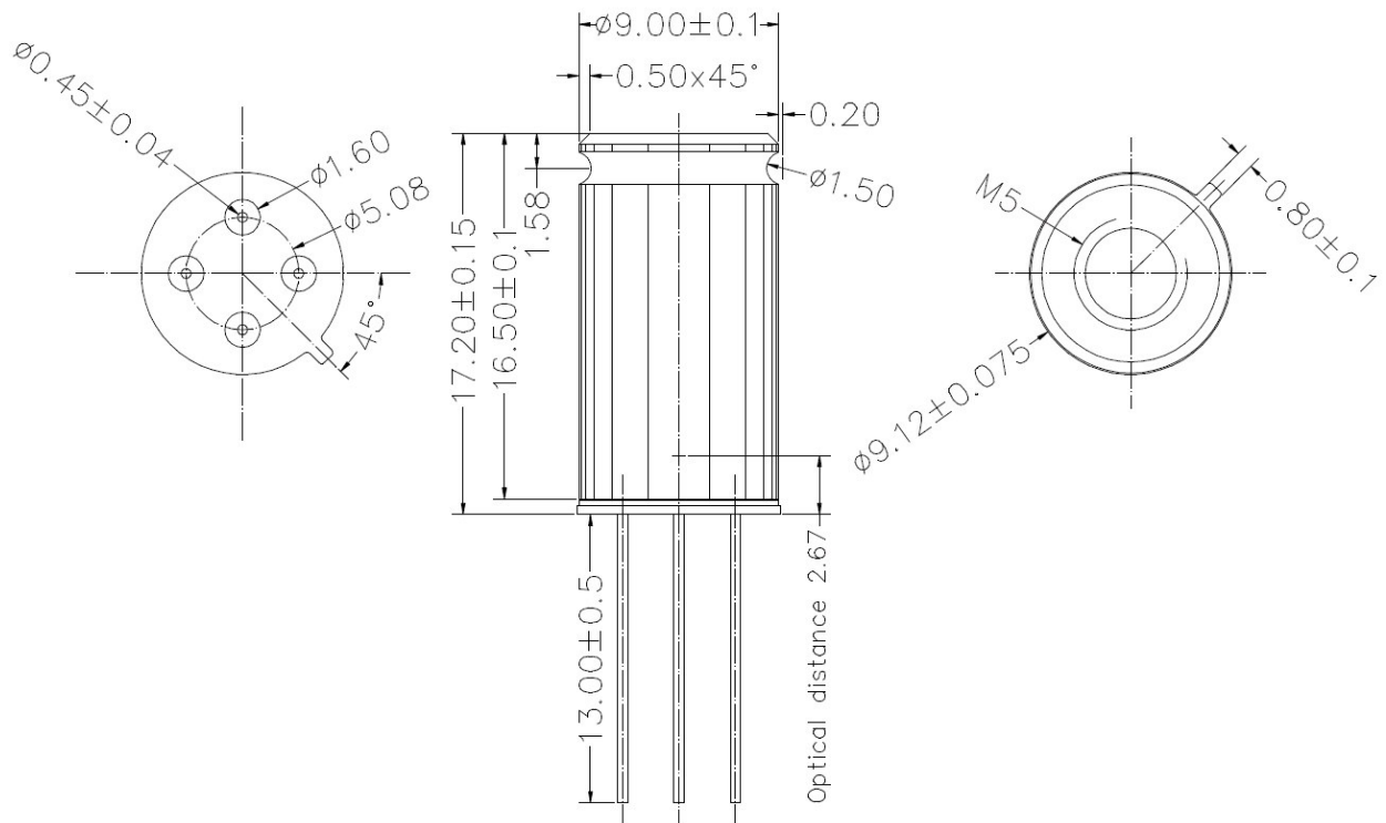
Figure 43: MLX90614xCF package
