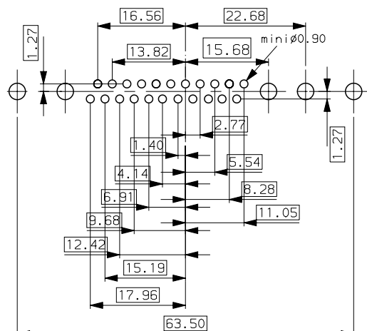
CONNECTOR SIDE VIEW
