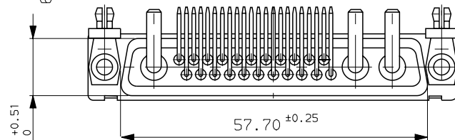
LAYOUT DIMENSIONS (after plating)
