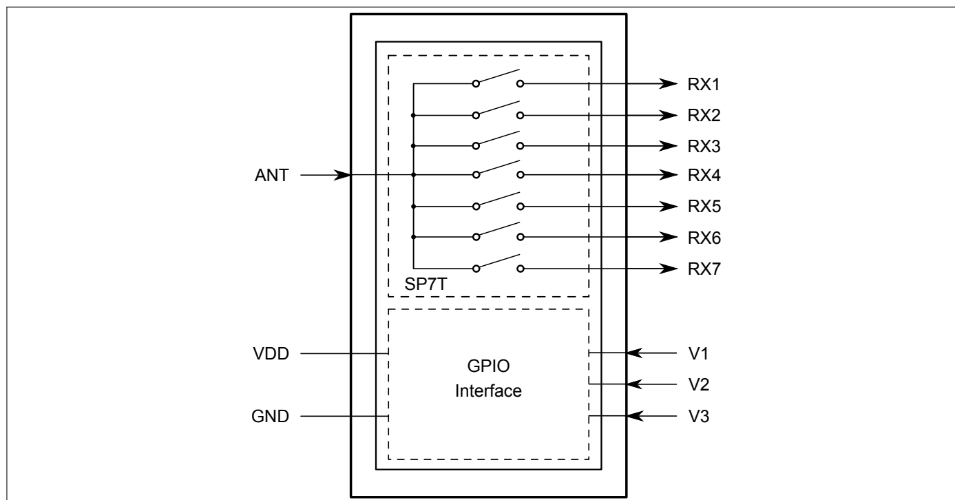
Figure 1: BGS17GA14 block diagram
