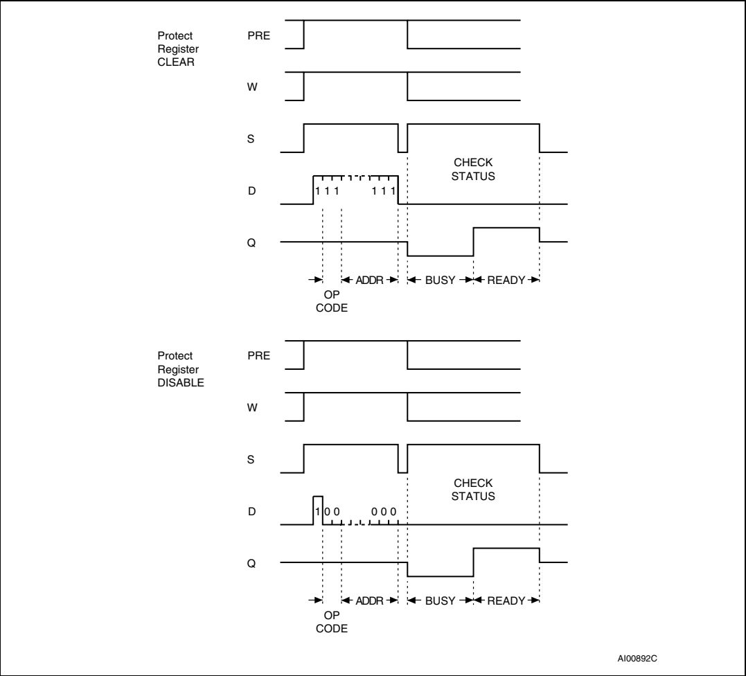
Figure 6. PRCLEAR and PRDS sequences
