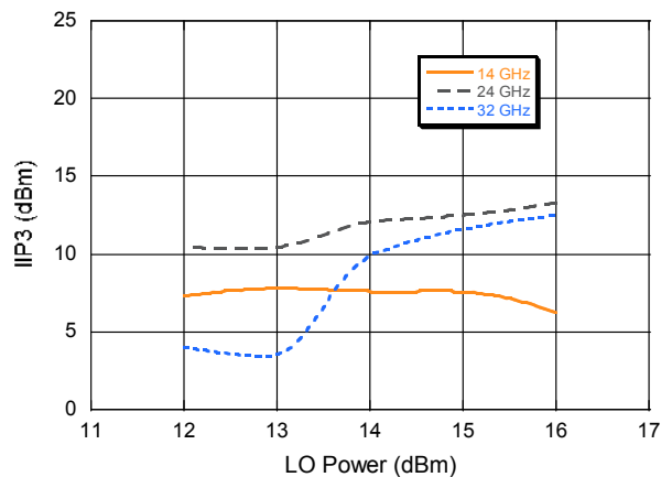
Up Conversion Input IP3 vs. LO Drive
