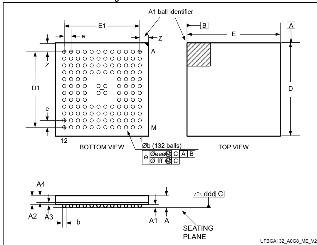
Figure 40. UFBGA132 outline
