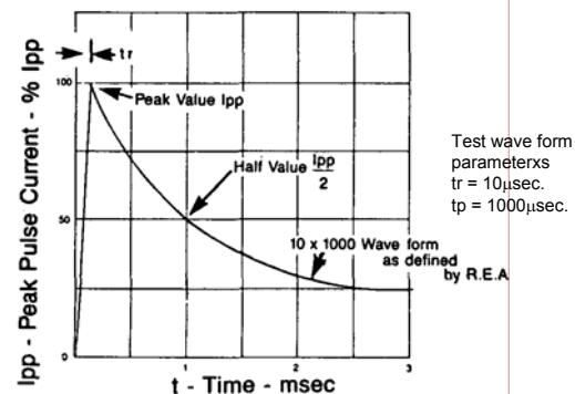
FIGURE 2 – PULSE WAVEFORM
