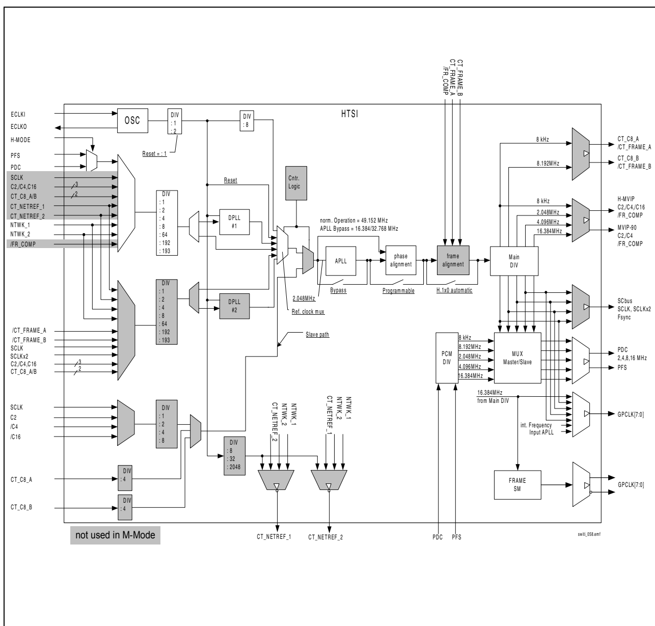
Figure 11 SWITI Clock Generator
