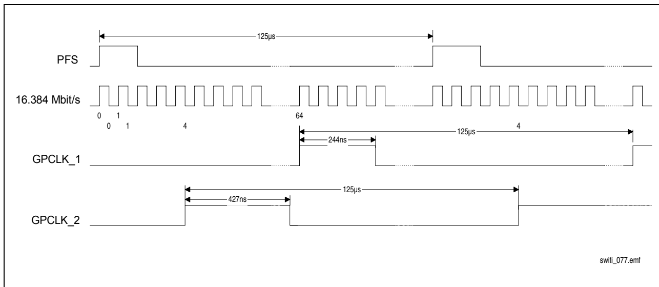
Figure 32 Example Framing Groups
