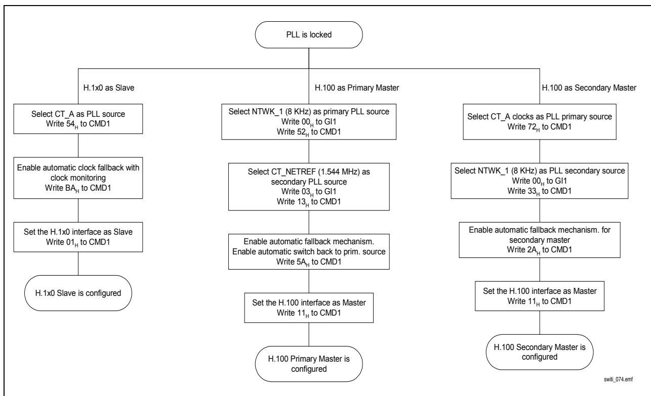
Figure 29 H.100 Master and Slave Configuration Process
