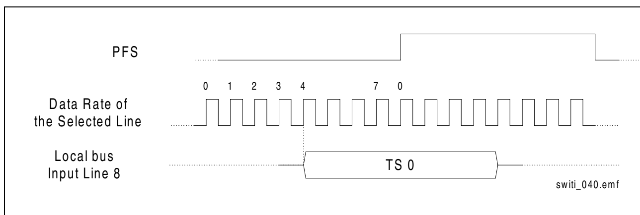
Figure 30 Example: Input Bit Shifting
