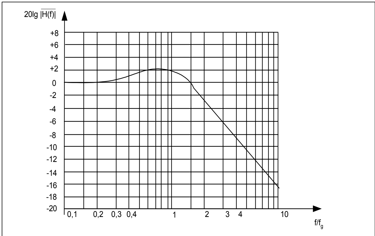
Figure 13 APLL - Jitter Transfer Function
