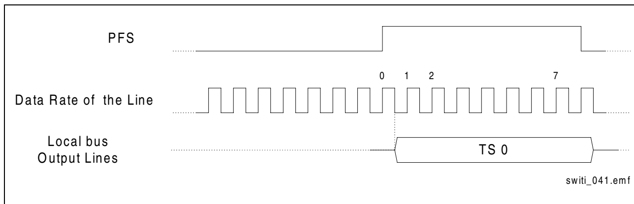
Figure 31 Example: Output Bit Shifting
