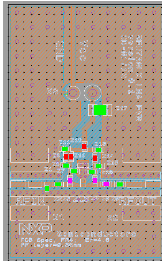
Fig 1. BFU730LX Universal Demo Board 5-5.9GHz WiFi LNA EVB Demo Board
